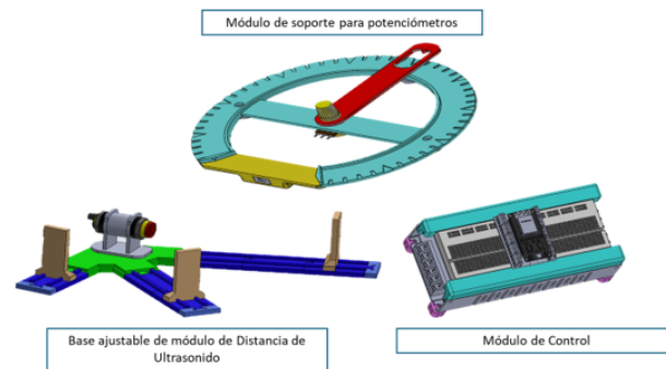
Figure 2. Physical sensor modules.
